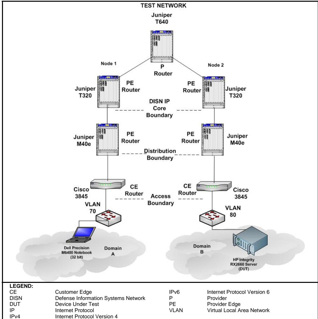
Figure 2-2. Test Network
