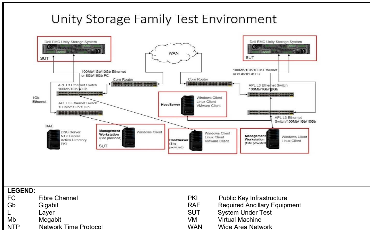
Figure 2-3. SUT Test Configuration
